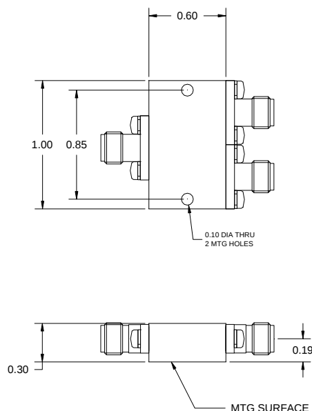
Small Outline
